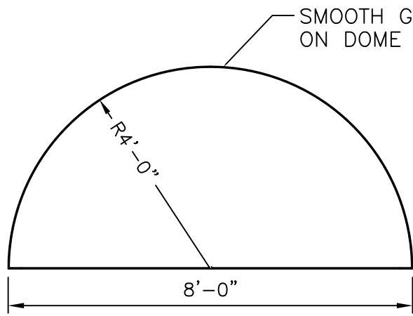
VERTICAL SECTION
